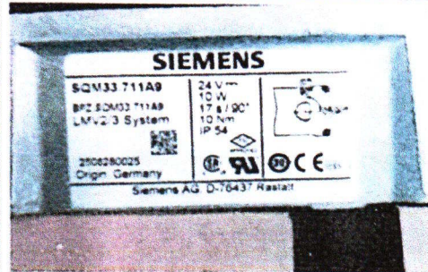
Diesel Burner Actuators Name Plate
