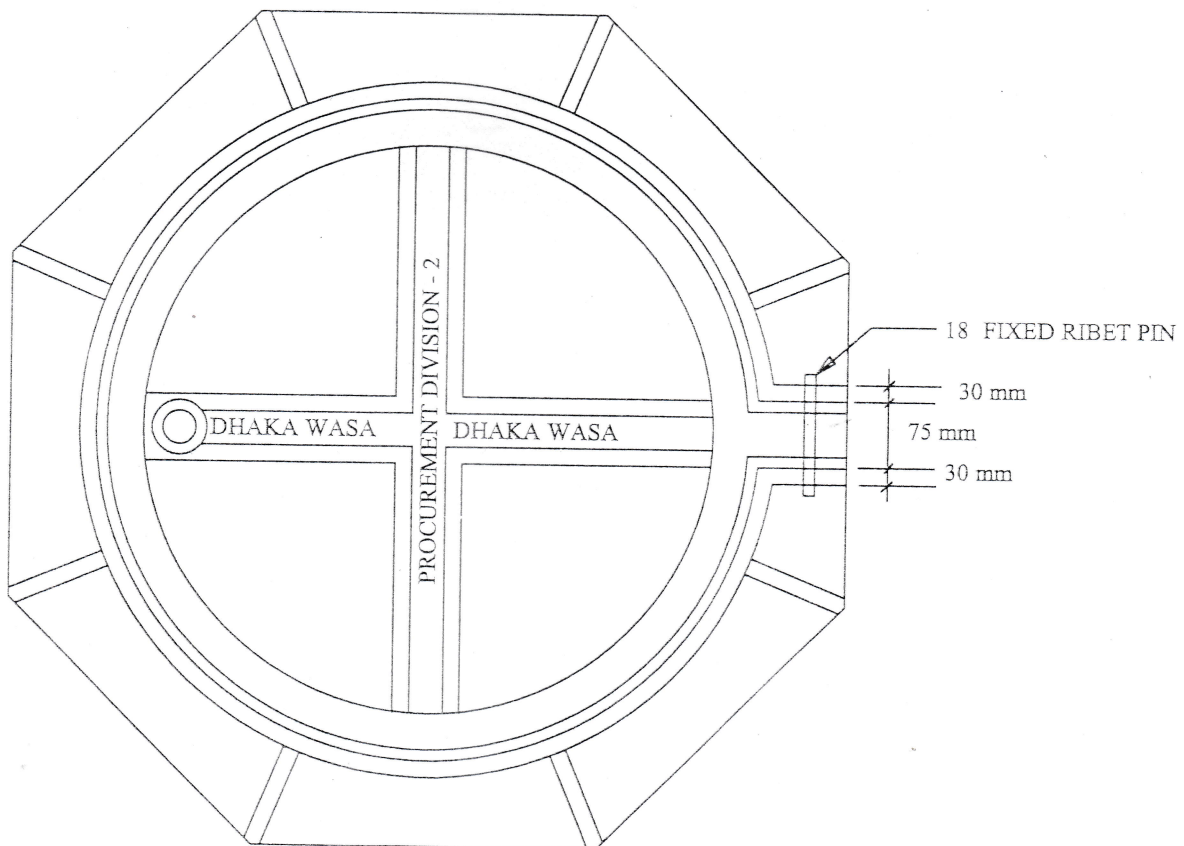
PLAN OF 550 mm DIA CI MANHOLE COVER
