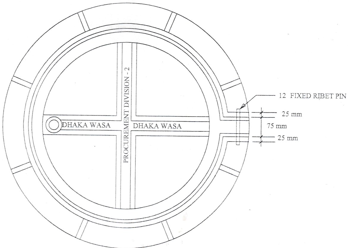
PLAN OF 450 mm DIA C.I. MANHOLE COVER NOT TO SCALE
